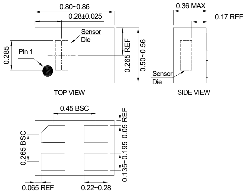
Fig.5 Outline package diagram of BBT-A908D0805 series sensor (unit: mm).
