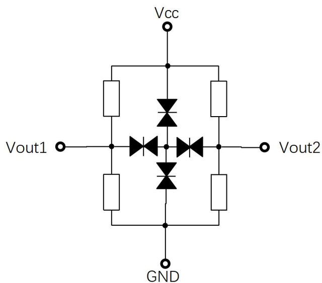
Fig. 2 Schematic diagram of the circuit of the BBT-A908D0805 sensor.
