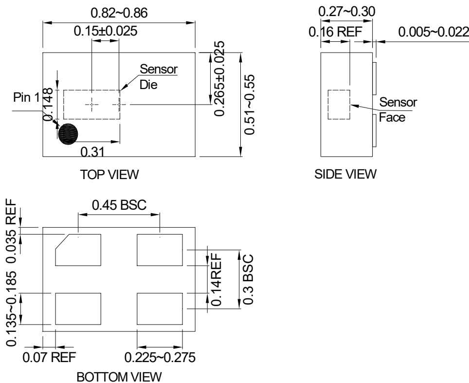
Fig.6 Outline package diagram of FFZ-001F58T22H series sensor (unit: mm).
